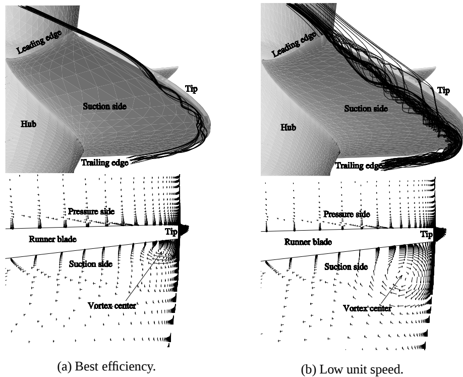
Figure 5: Comparison between the tip vortex size and location at the best efficiency operating condition and at a lower unit speed. The vectors are located in a meridional plane at the center of a runner blade and are projected in the main flow direction in order to magnify the secondary flow.
