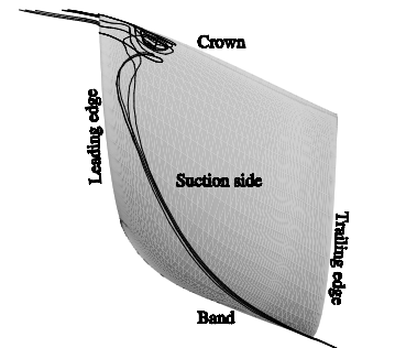
(f) Re-circulation at the leading edge suction side, close to the crown. Operating point 4.
