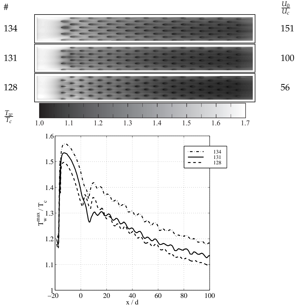
Figure 5.7: The effect of different velocity ratios, U_0/U_c , is shown in thermo-graphs of a teflon plate where T_0/T_c=1.7 , Re_c=92 , \delta x/d=6 , \alpha=20^\circ and n=80 . A variation in U_0/U_c is made, from top U_0/U_c=\{151, 100, 56\} . (Reprinted with the permission of ASME.)
