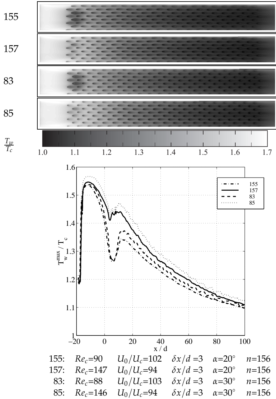
Figure 5.10: The effect of different Reynolds numbers, Re_c , is shown in thermographs of a teflon plate where T_0/T_c=1.7 . (Reprinted with the permission of ASME.)
