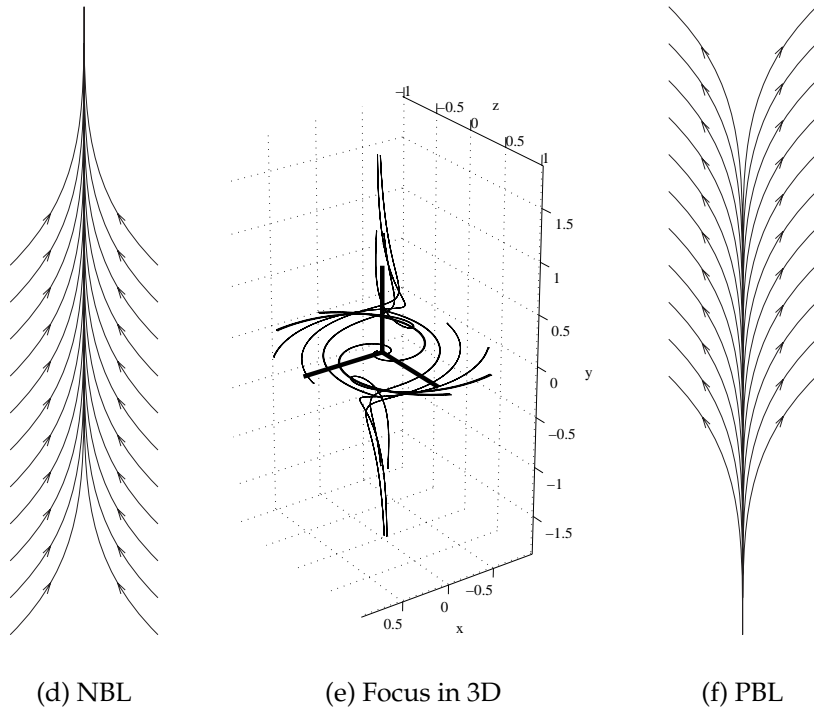
Figure 9.1: Figures (a) through (c) show three different kinds of critical points. In (e) a focus with one real and two complex conjugate eigenvalues \lambda_1 = 0.5 , \lambda_{2,3} = 0.5 \pm i , is drawn. Figure (d) shows a negative bifurcation line, i.e. a separation line , and figure (f) a positive bifurcation line, i.e. an attachment line .
