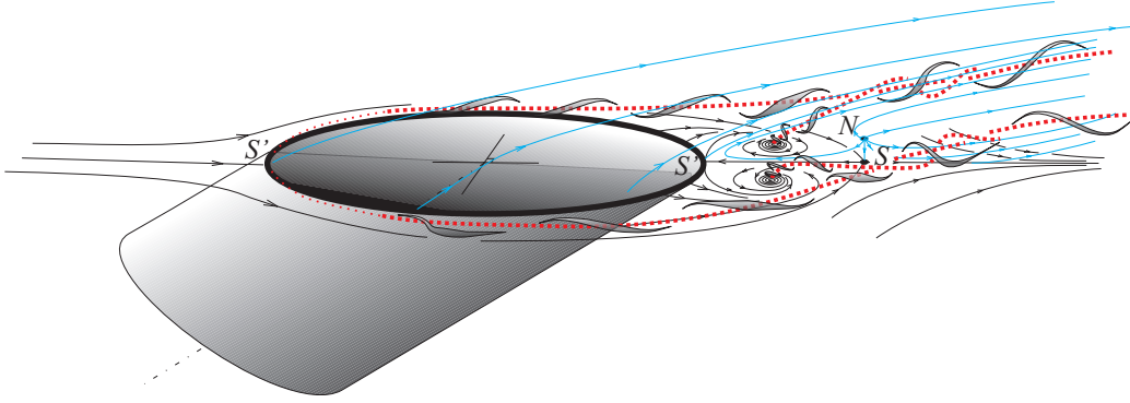
Figure 9.3: Interpretation of the measured velocity field and its topology.
