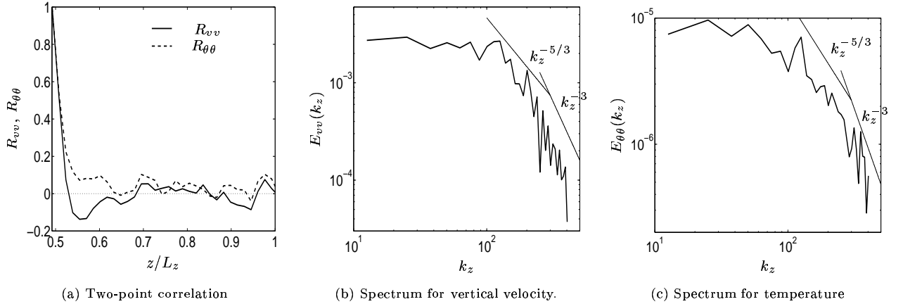
Figure 8: Spanwise two-point correlation and one-dimensional energy spectra for vertical velocity and temperature (at x/L_x \approx 0.028 , y/L_y \approx 0.5 and z/L_z \approx 0.492 , with Case D).
